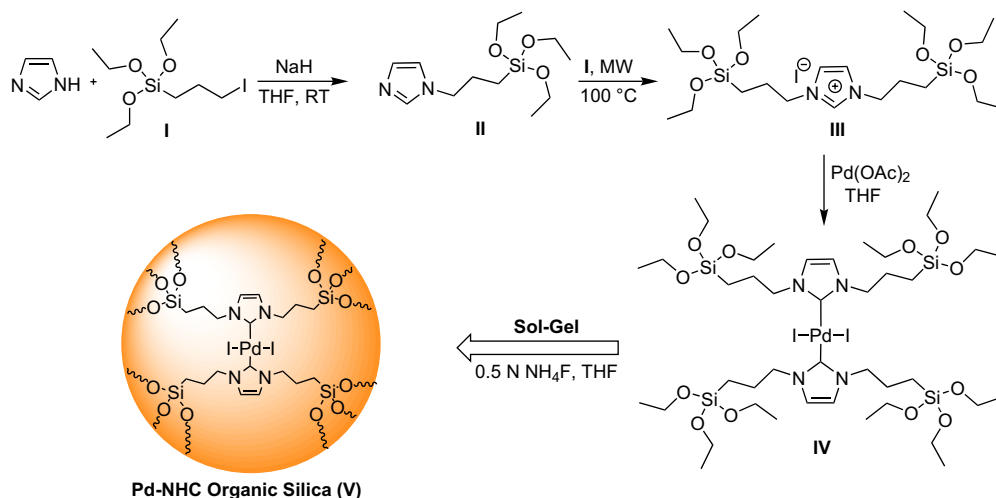
Scheme 1. Preparation of Pd– N -heterocyclic carbene (NHC) organic silica.
