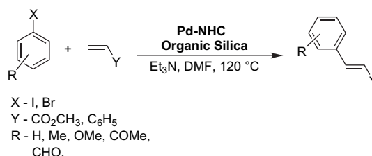
Scheme 2. Heck reaction using Pd– N -heterocyclic carbene organic silica.
